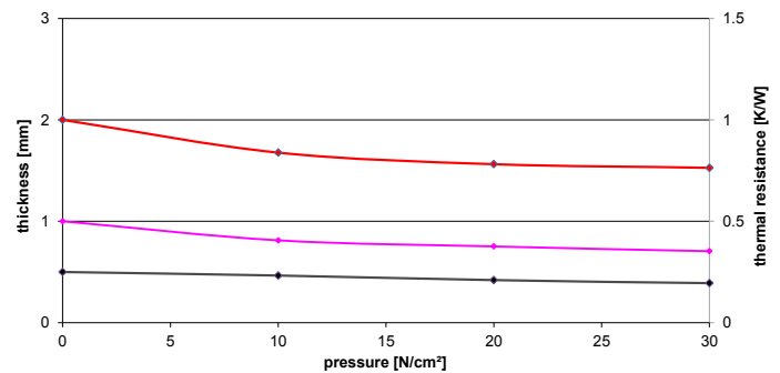
Compression 86/500
