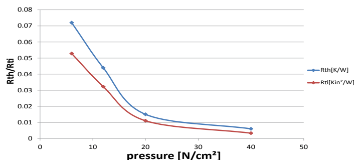
Compression KP 12
