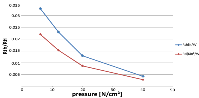
Compression KP 99
