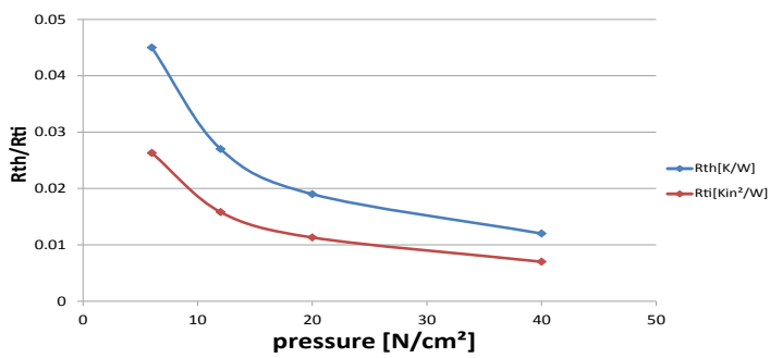
Compression KP 97
