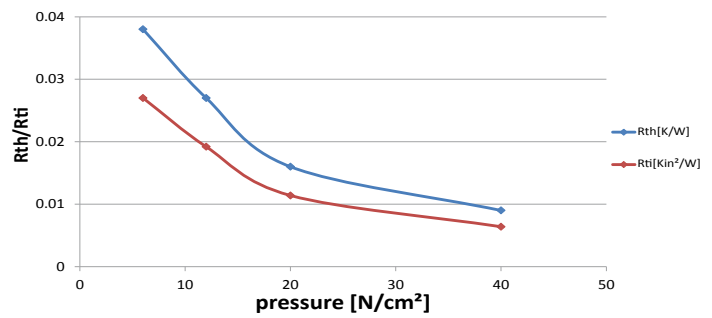
Compression KP 98
